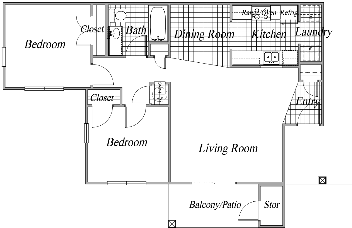
Milburnie Place 2 Bedroom Plan - 863 SF
